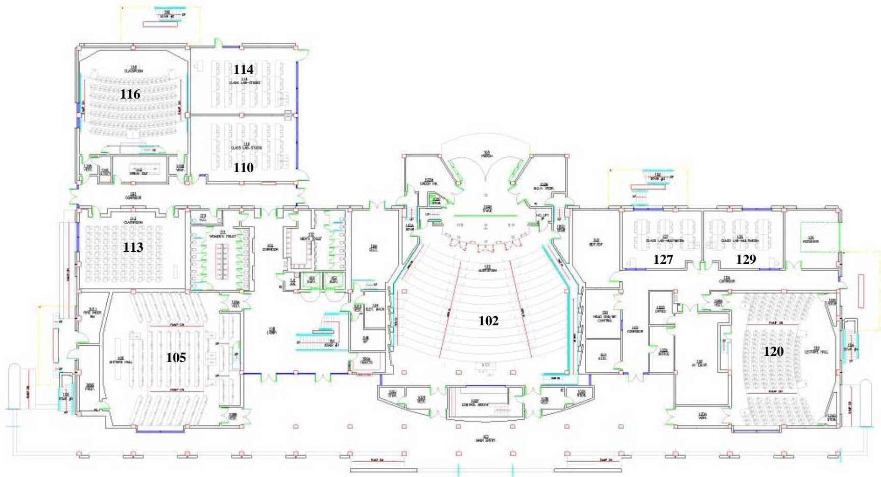
Classroom and Office Building First Floor
